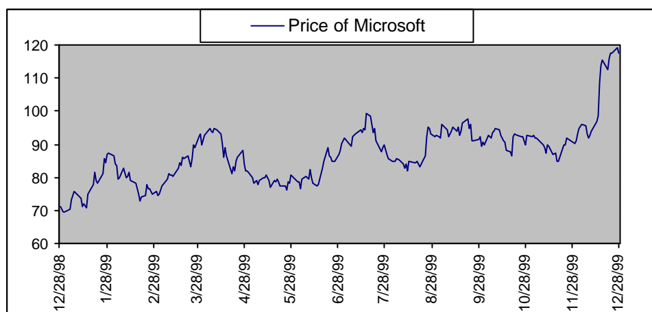
Figure 1: The price movement of Microsoft
